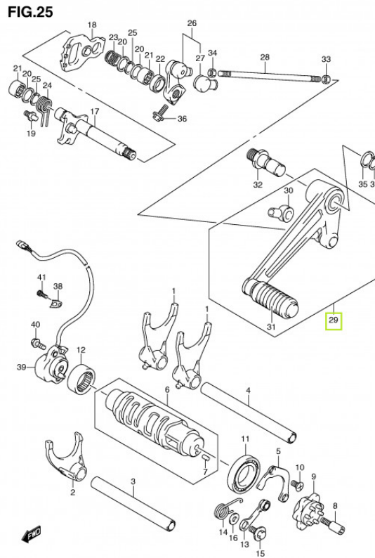
GSX1300RKB E02_025 GEAR SHIFTING-C
