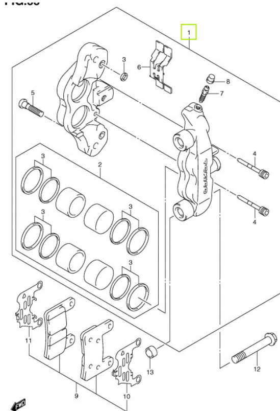
GSX1300RK8 E02_055 FRONT CALIPER-C
