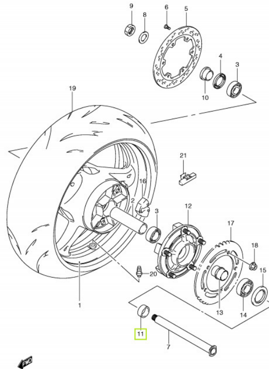
GSX1300RK8 E02_060 REAR WHEEL-C
