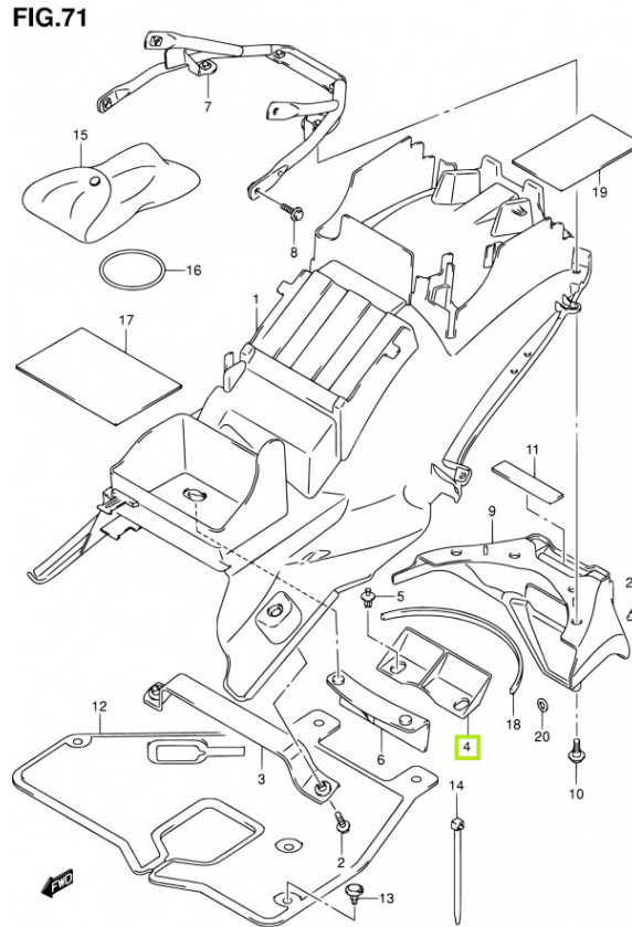
GSX1300RAL4_E02_071 REAR FENDER
